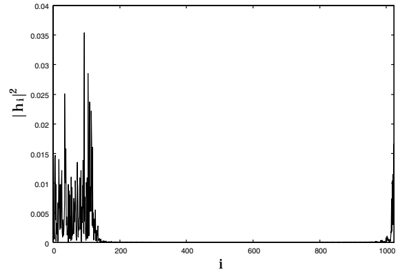
Fig. 3. Delay power spectrum: simulation.
