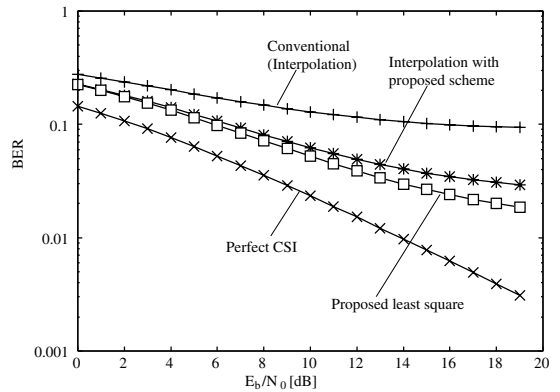
Fig. 4. BER performance (# of pilot subcarriers: 256).
