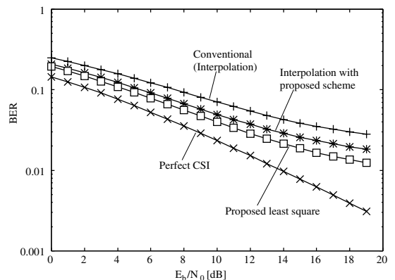
Fig. 5. BER performance (# of pilot subcarriers: 512).
